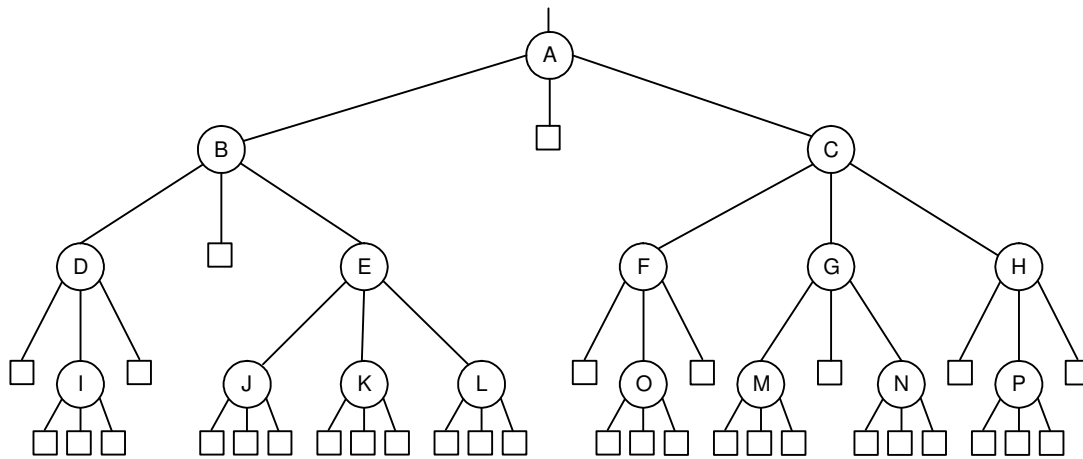
Fig. 4.19. Ternary tree extended with special nodes
