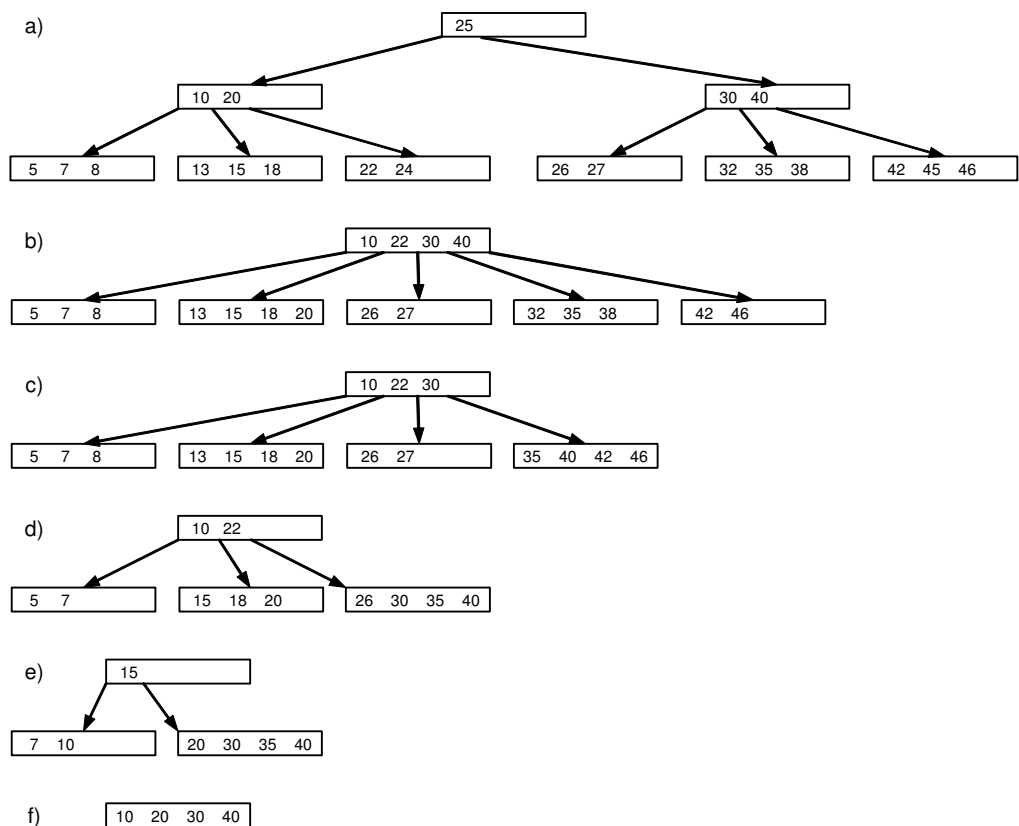
Fig. 4.46. Decay of B-tree of order 2
