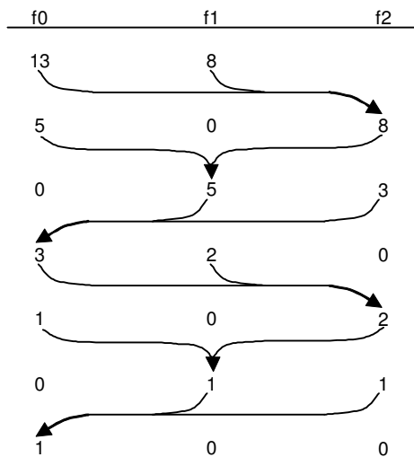
Fig. 2.14. Polyphase mergesort of 21 runs with 3 sequences
