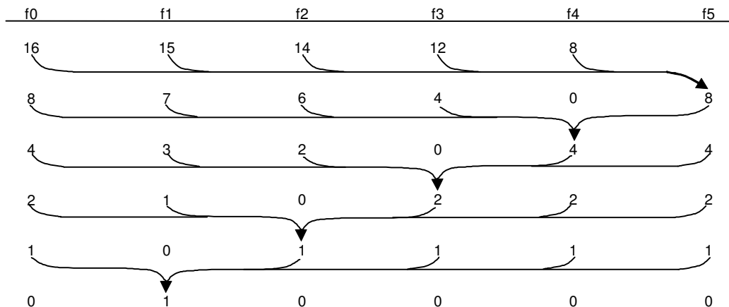
Fig. 2.15. Polyphase mergesort of 65 runs with 6 sequences
